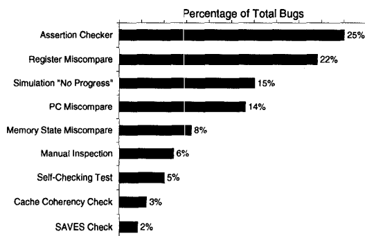
Figure 6. Bug Detection Mechanisms
