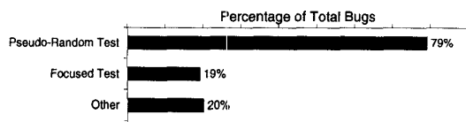
Figure 4. Effectiveness of Test Category
