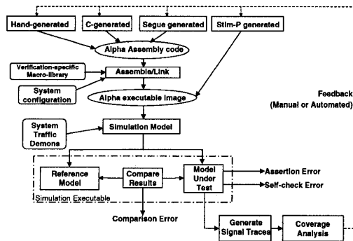
Figure 1. Verification Test Environment
